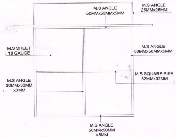
STRUCTURE DRAWING
