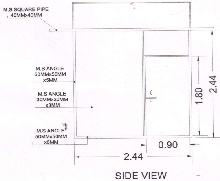
MILK PARLOUR SIDE VIEW
