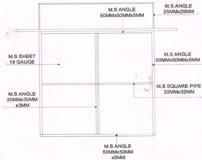
STRUCTURE DRAWING
